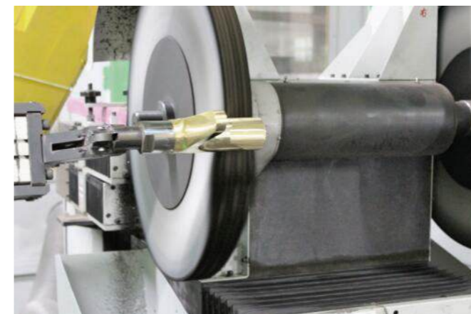
Robotic polishing to guarantee a perfect finish on product
