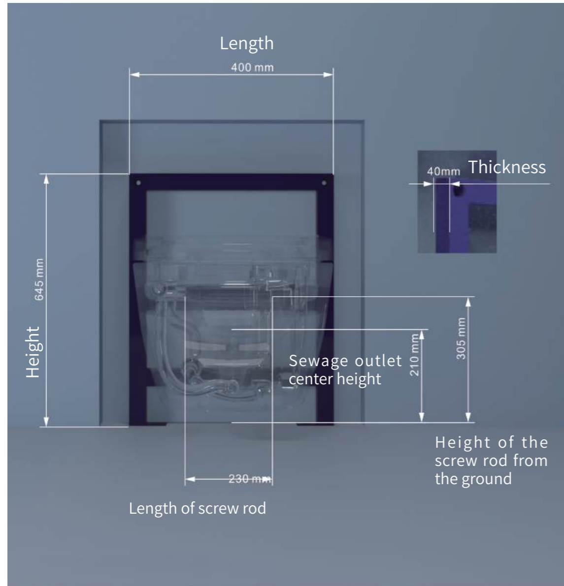
Size of tank support (WS-28X, WS-02)
