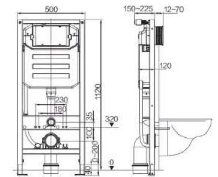
Tank support height : 820/1120mm
