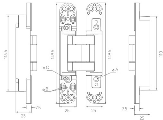
A: Front and rear adjustment B: Adjust up and down C: Left and right adjustment
