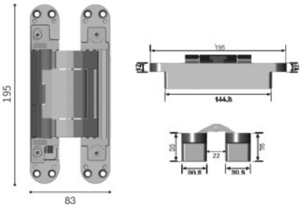
Functional diagram
