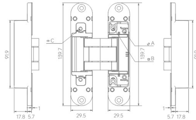
A: Front and rear adjustment B: Adjust up and down C: Left and right adjustment
