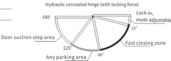
Functional diagram
