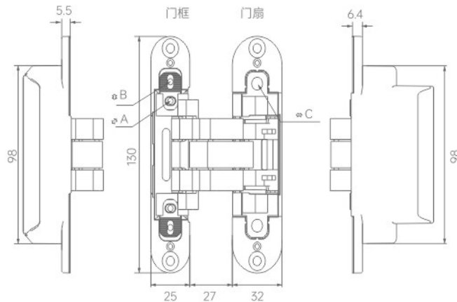
A: Front and rear adjustment B: Adjust up and down C: Left and right adjustment
