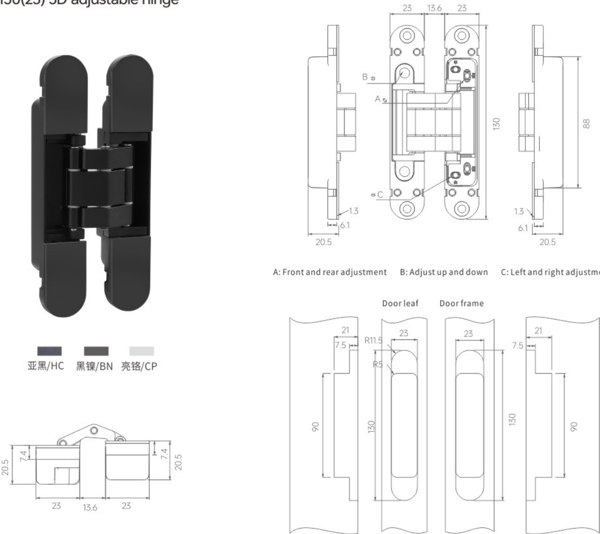
HE3D130(23) 3D adjustable hinge
